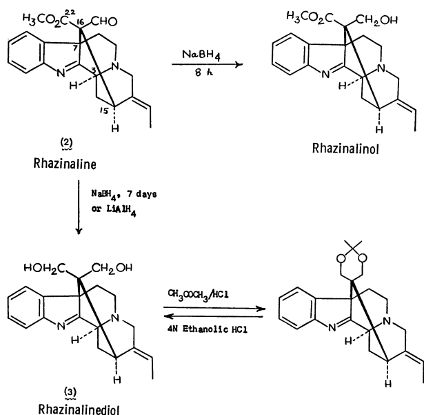
Chart 2. Reaction of rhazinaline.
